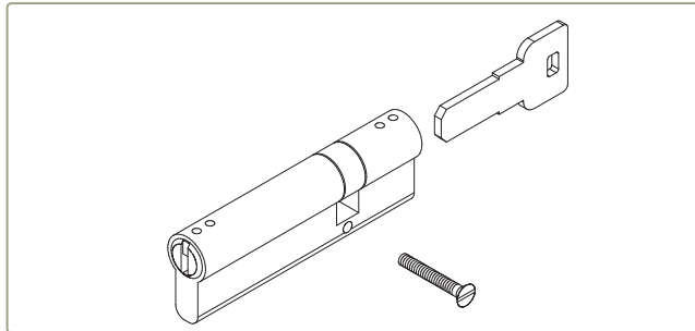
207401 CILINDRO BKS 80/50
